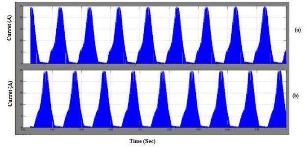
Fig.3.5. Output inductor current (a)ilo1=28A (b) ilo1=28A.
