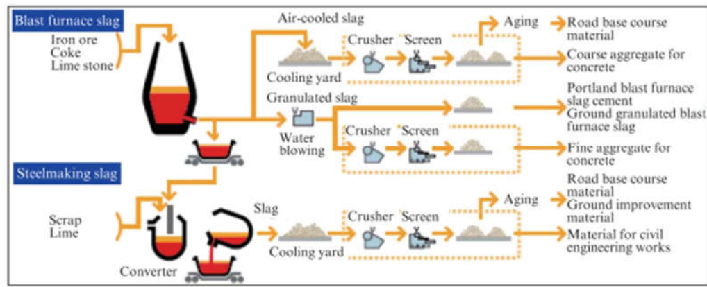
Fig. 5. Steel Slag Recycling in road construction
