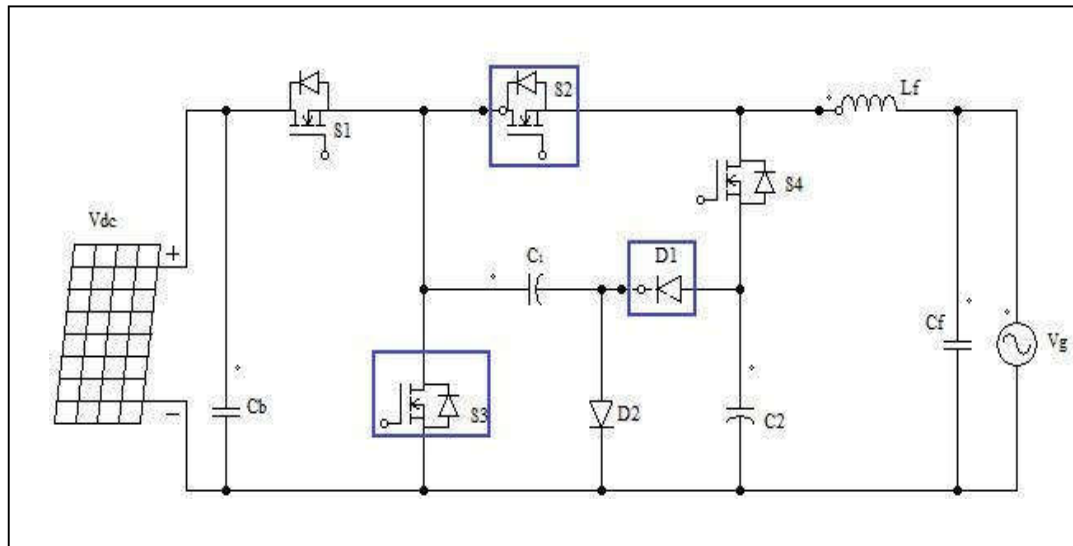
Figure 7: Proposed SST inverter topology during (i) first half period (ii) zero state and (iii) second half period.
