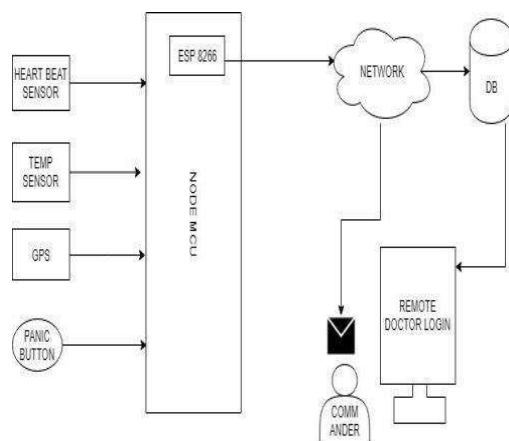
FIG.SOLDIER HEALTH MONITORING & TRACKING SYSTEM USING IOT
