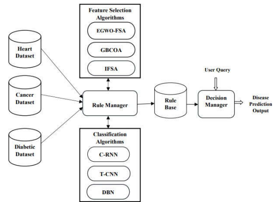
Figure 3.2 Workflow of Proposed Disease Prediction System
