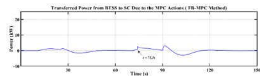
Fig (10). Transferred power from BESS to SC because of the MPC actions in the FB-MPC method.
