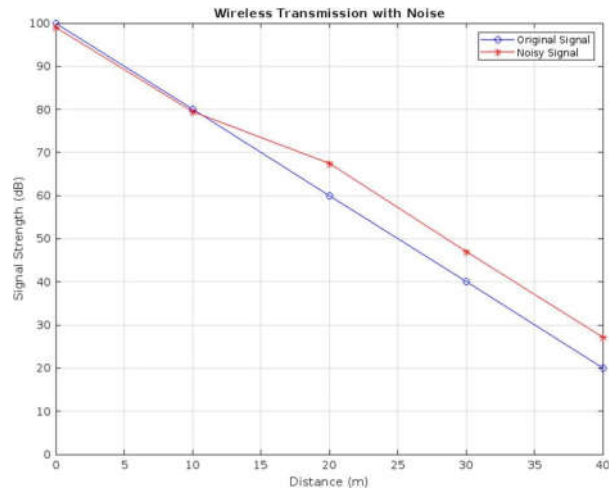
Fig2: Wireless data transmission.
