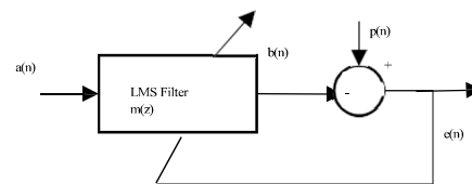
Figure 3.2: Structure of adaptive filter
