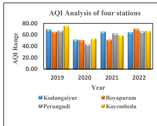
Figure 2. Analysis of AQI data
