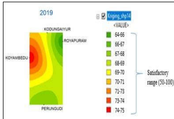
Figure 7. Kriging model for the year 2019
