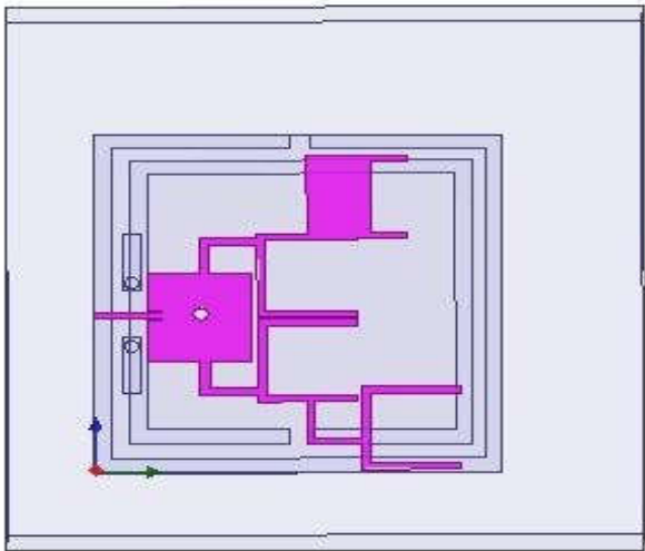
Figure 2 Micro strip patch array filter
