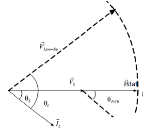
Fig.3. Phasor diagram of IPC Method
