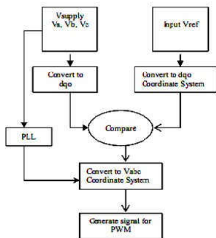
Fig.4. Feed forward control Technique for DO_0 transformation
