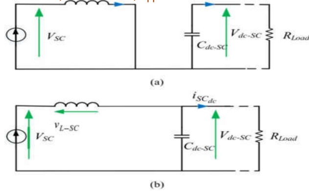
FIGURE 5. Electrical scheme of a buck-boost converter. a) Active phase b) Freewheeling phase
