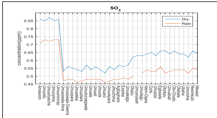
Fig. 17: Sulphur Dioxide MATLAB Comparison Model
