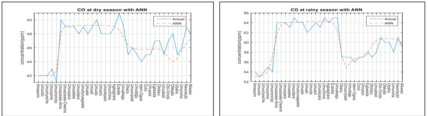
Fig. 7 Comparative Analysis of Actual and Predicted CO
