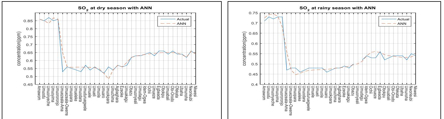
Fig. 19: Comparative Analysis of Actual and Predicted SO 2
