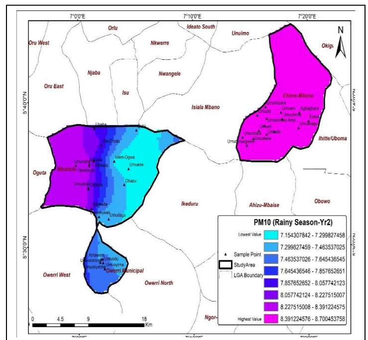
PM 10 at Rainy Season Year 2
