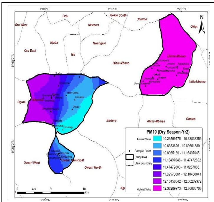
PM 10 at Dry Season Year 2
