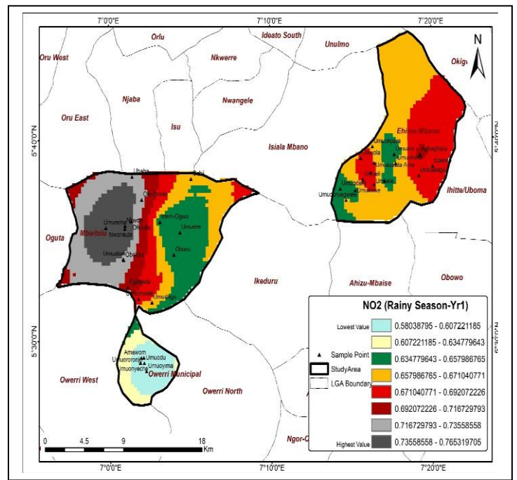
NO 2 at Rainy Season Year 1
