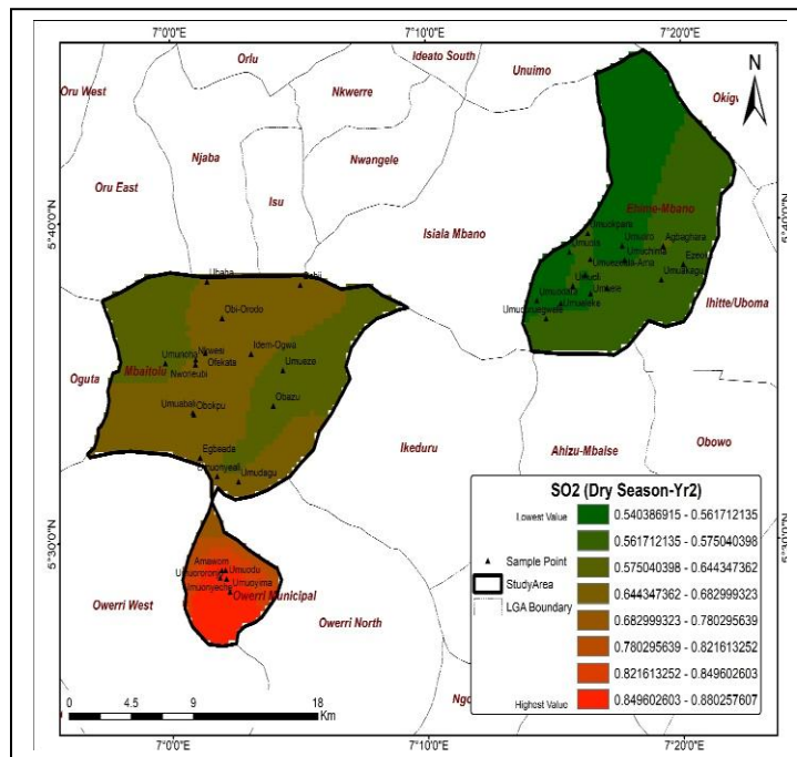
SO 2 at Dry Season Year 2
