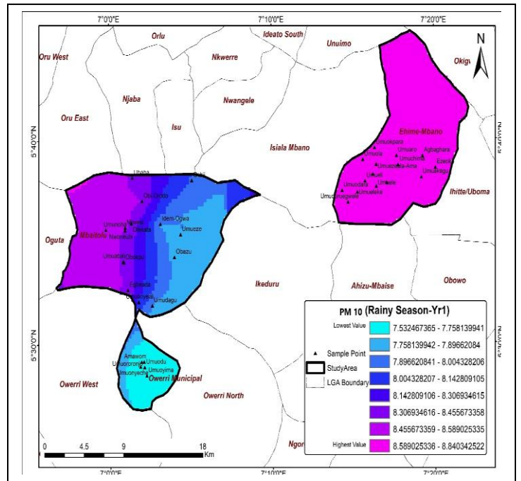
PM 10 at Rainy Season Year 1
