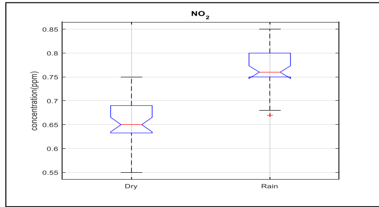
Fig. 14 Nitrogen Dioxide Box & Whiskers Comparative Plot Dry and Rainy Seasons
