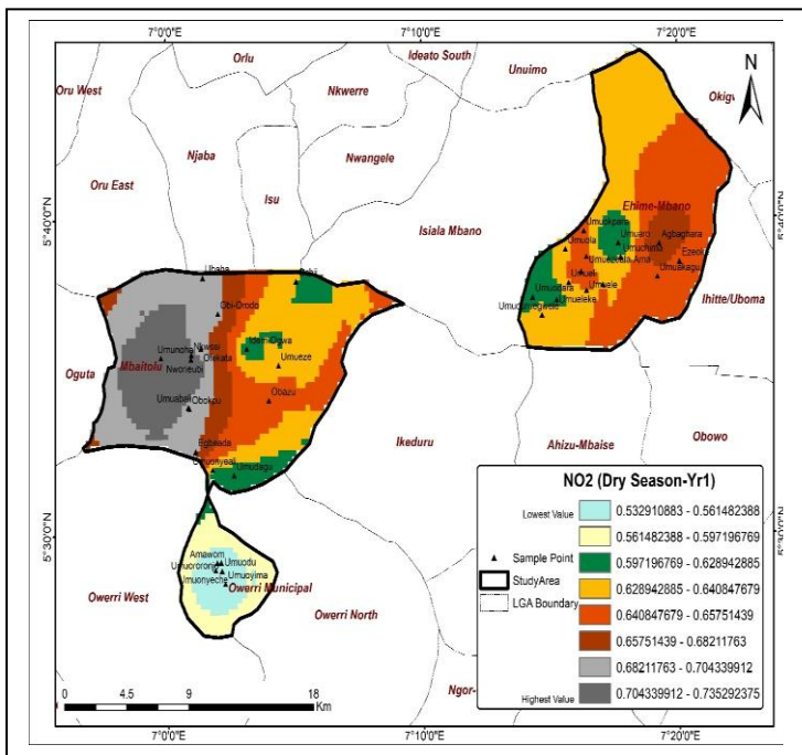
NO 2 at Dry Season Year 1
