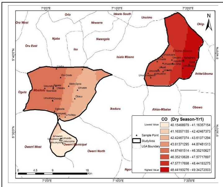
CO at Dry Season Year 1
