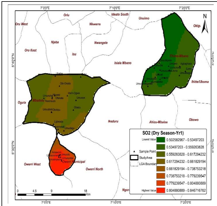
SO 2 at Dry Season Year 1
