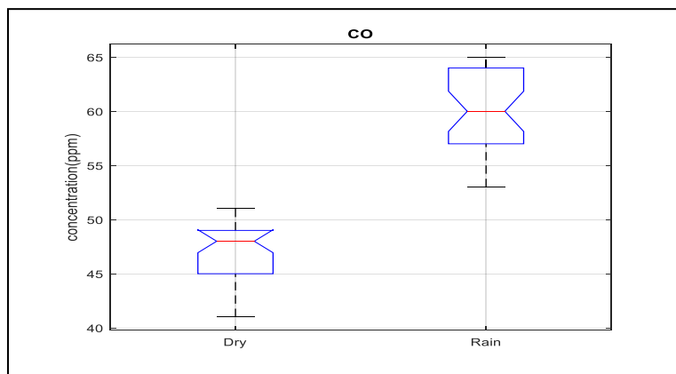
Fig. 8 Carbon Monoxide Box & Whiskers Comparative Plot Dry and Rainy Seasons.
