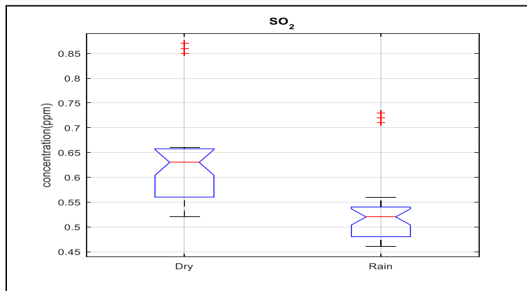
Fig. 20: Sulphur Dioxide Box & Whiskers Comparative Plot Dry and Rainy Seasons
