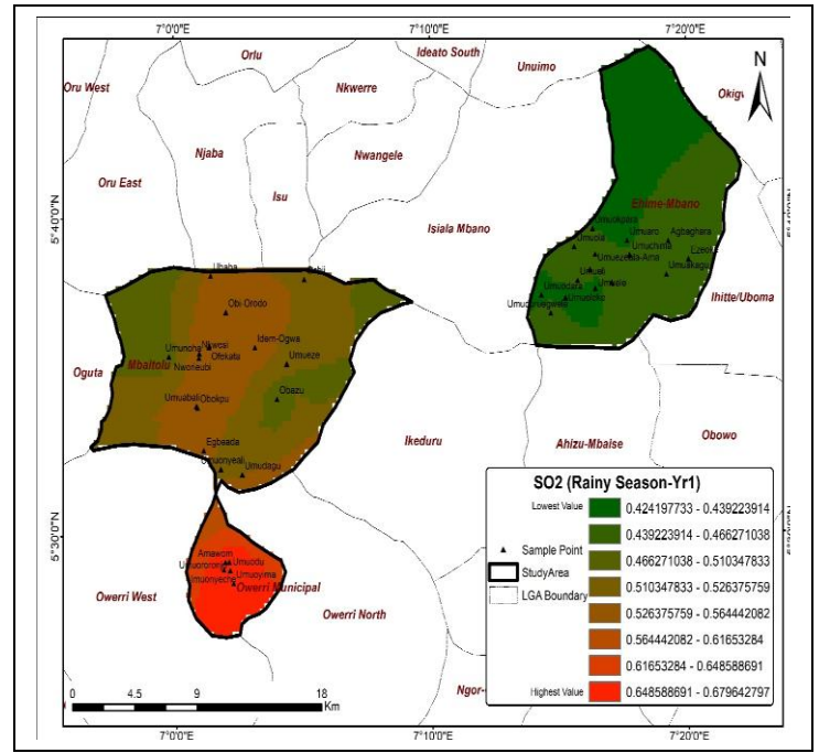
SO 2 at Rainy Season Year 1
