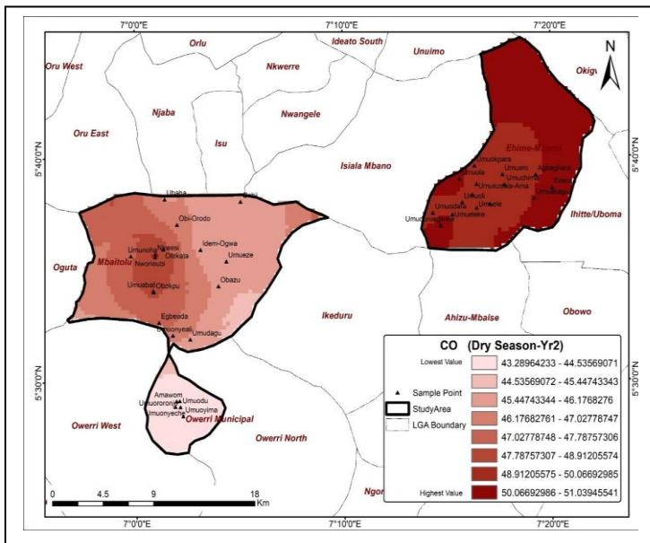
CO at Dry Season Year 2
