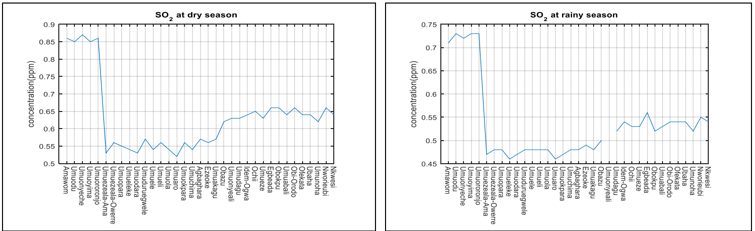
Sulphur Dioxide at Dry Seasons
