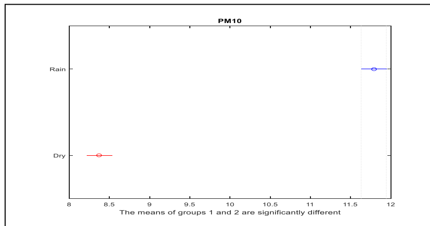
Fig. 27: Particulate Matter Mean Comparative Analysis Dry and Rainy Seasons
