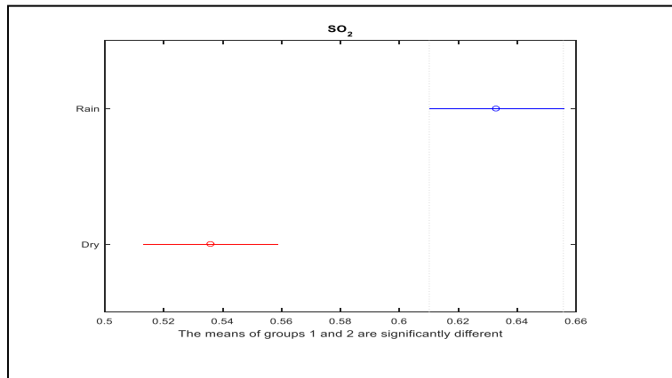
Fig. 21: Sulphur Dioxide Mean Comparative Analysis Dry and Rainy Seasons
