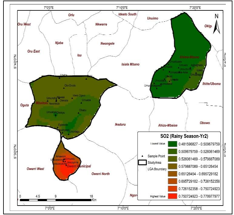
SO 2 at Rainy Season Year 2
