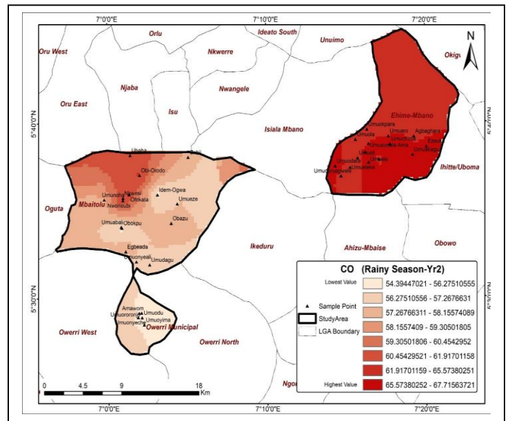
CO at Rainy Season Year 2
