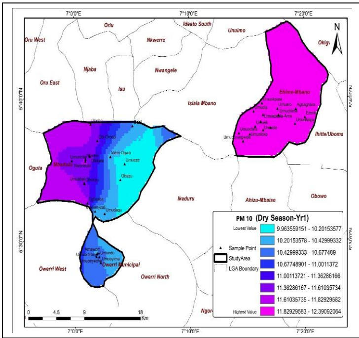
PM 10 at Dry Season Year 1
