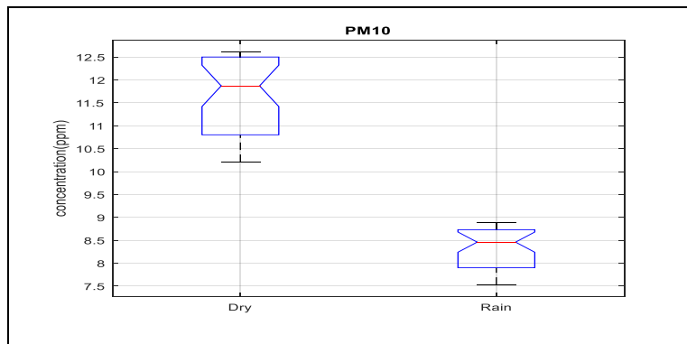
Fig. 26: Particulate Matter Box & Whiskers Comparative Plot Dry and Rainy Seasons
