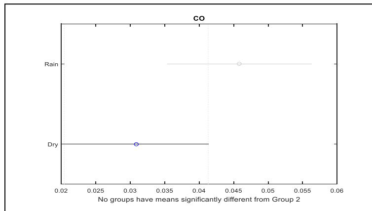
Fig. 9 Carbon Monoxide Mean Comparative Analysis Dry and Rainy Seasons
