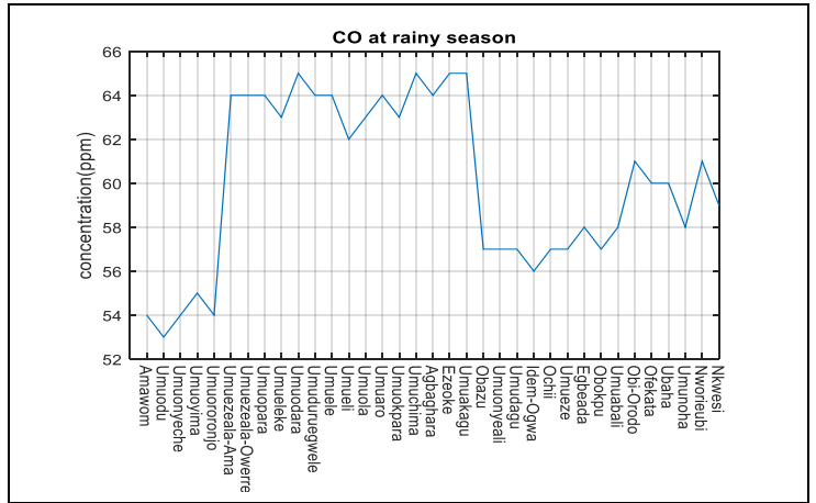
Carbon Monoxide at Rainy Seasons
