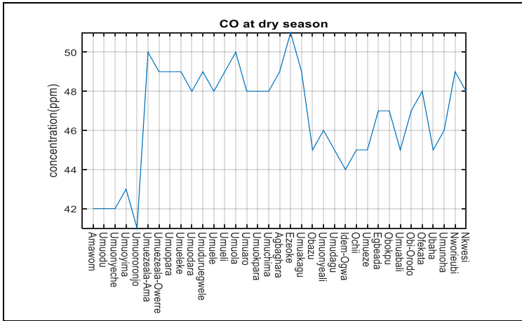
Carbon Monoxide at Dry Seasons
