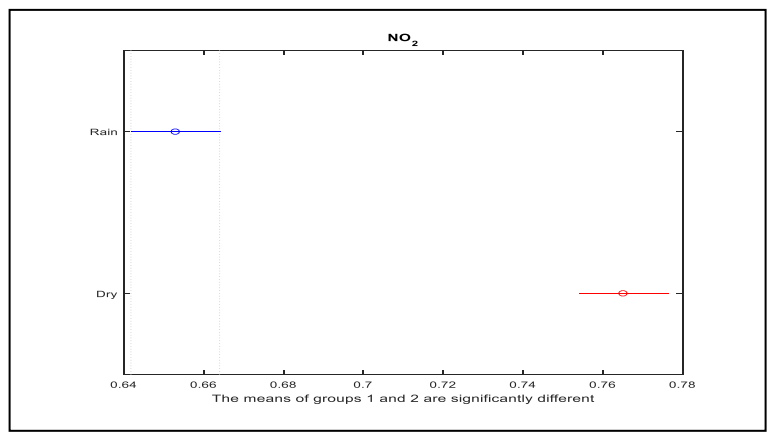
Tab Fig. 15: Nitrogen Dioxide Mean Comparative Analysis Dry and Rainy Seasons
