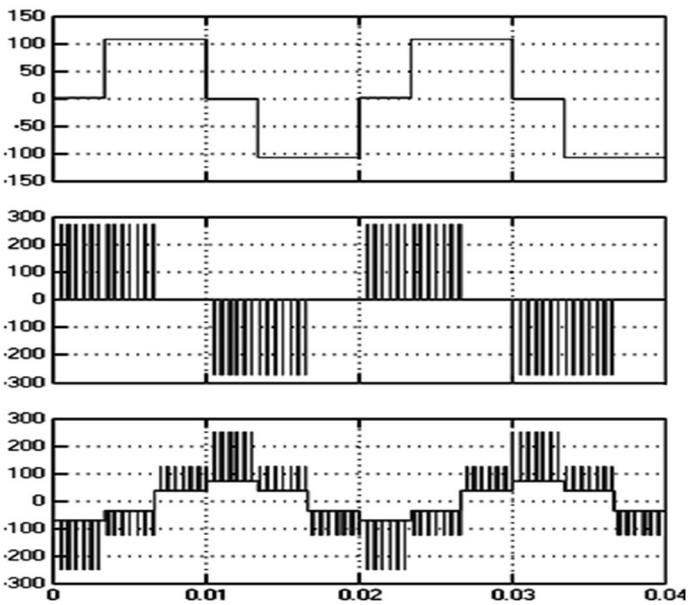
Figure14 Output waveform for layer 3
