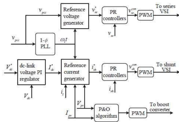
Fig.2.1. Overall control diagram of single-phase SPV-UAPF system.
