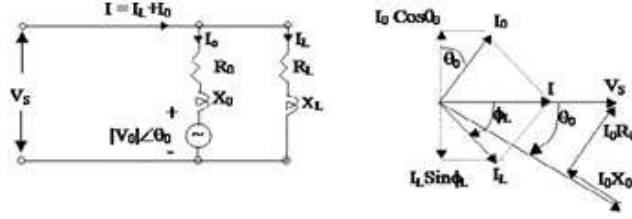
Fig.1. Inductive mode of operation
