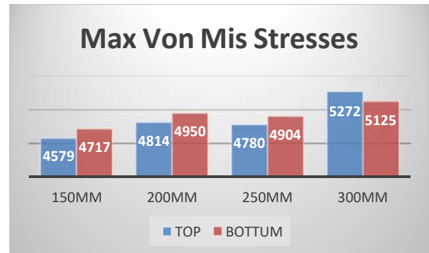
Graph.5: Max von mis Stresses on Deck Slab of 15m Span with varying thickness
