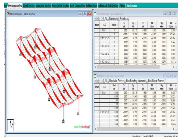
Fig 3: Stresses on Deck Slab
