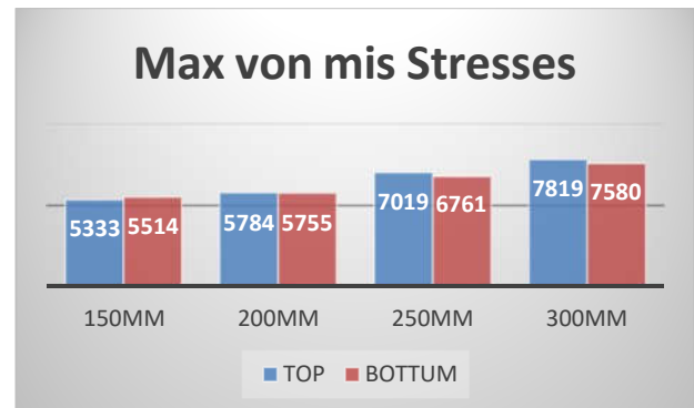
Graph.6: Max von mis Stresses on Deck Slab of 18m Span with varying thickness
